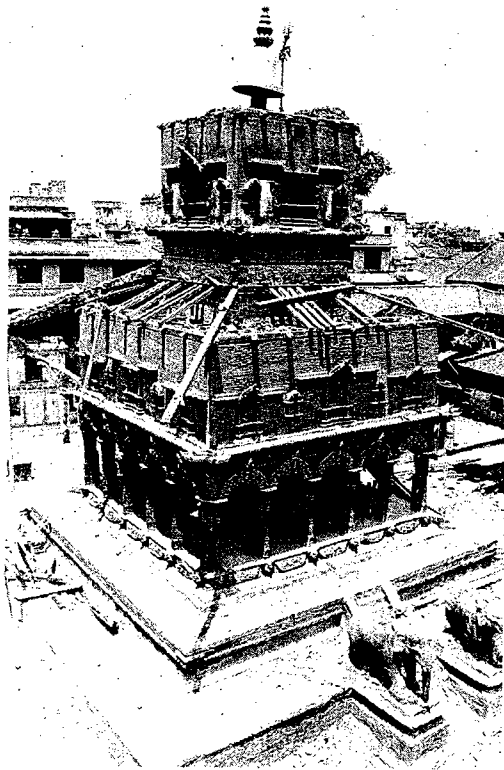
Fig. 2--Viswanath Temple, after collapse
